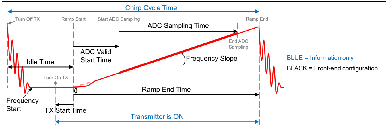
Figure 2: Chirp Diagram
