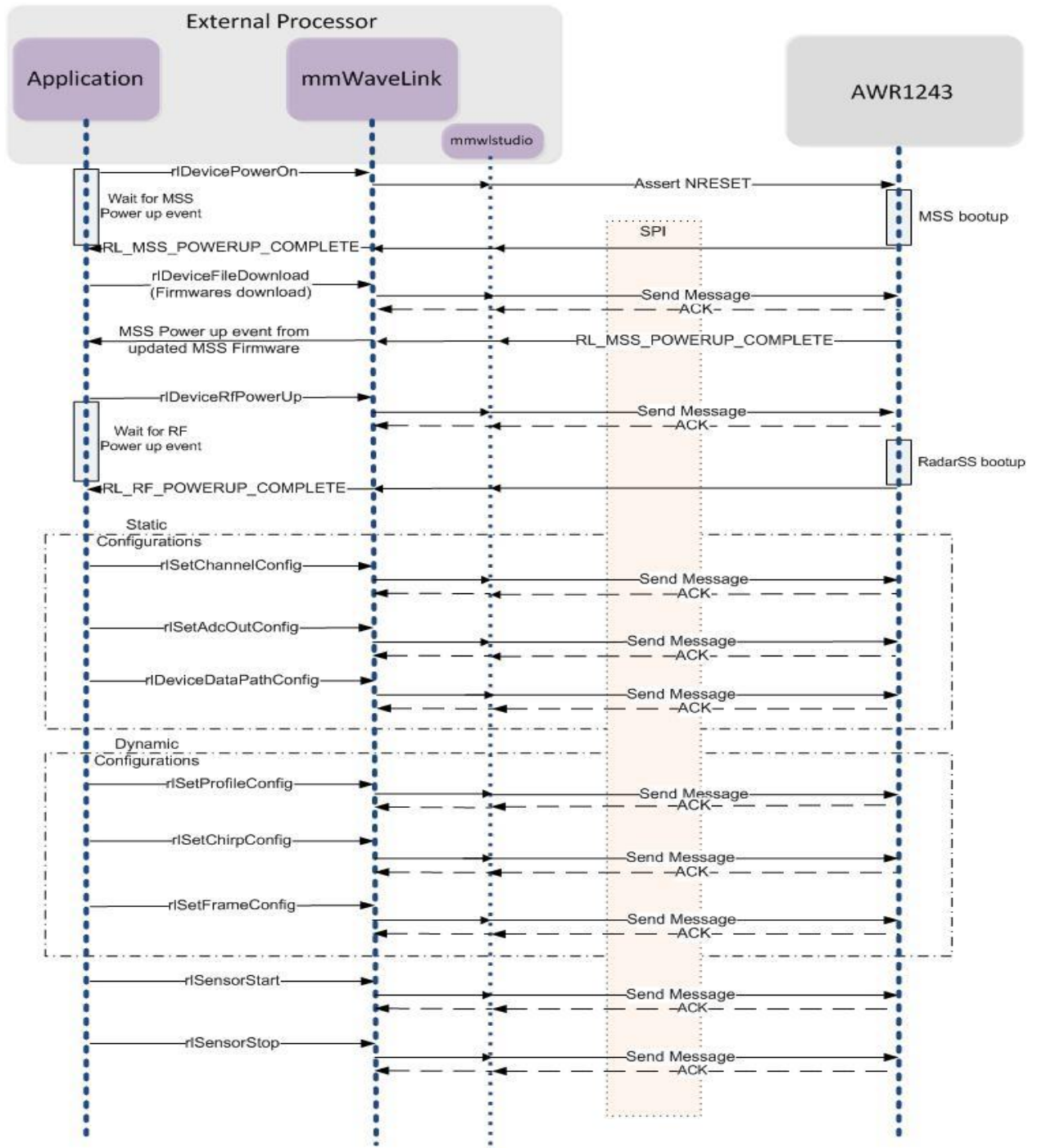
Figure 13. API Sequence
