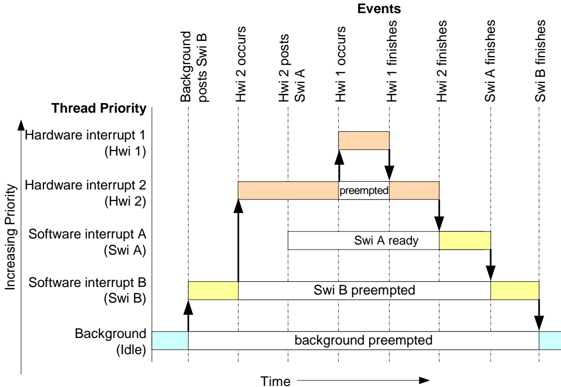
Figure 2-2. Preemption Scenario
