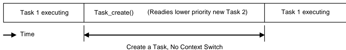
Figure C-6 Create a New Task without Context Switch
