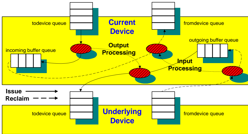
Figure 7–14 Copying Stacking Driver Flow
