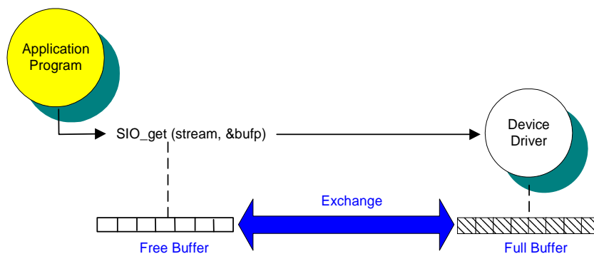
Figure 7–3 How SIO_get Works
