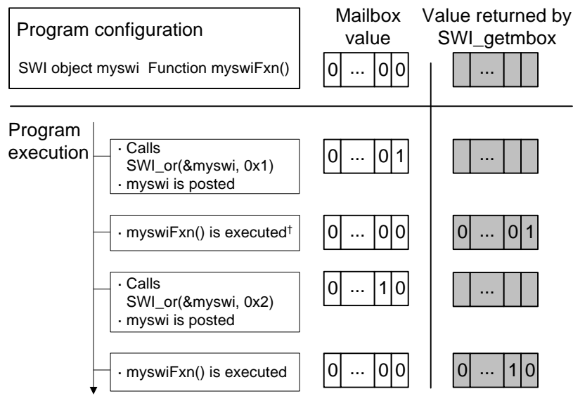
Figure 4–9 Using SWI_or to Post an SWI.
