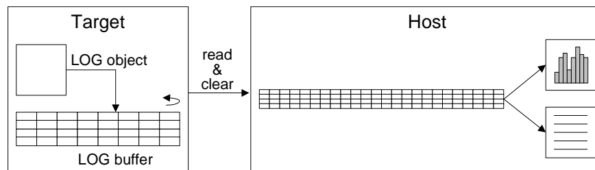
Figure 3–1 LOG Buffer Sequence
