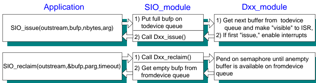
Figure 7–9 Placing a Data Buffer to a Stream
