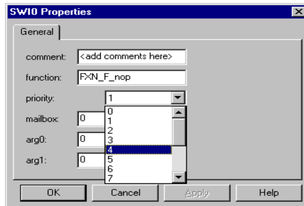
Figure 4–6 SWI Properties Dialog Box
