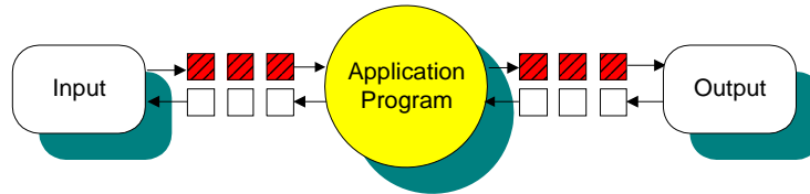
Figure 6–1 Input/Output Stream
