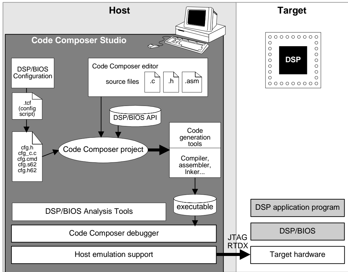
Figure 1–1 DSP/BIOS Components
