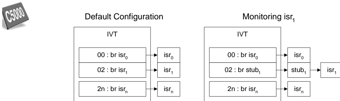
Figure 3–5 Monitoring Stack Pointers (C5000 platform)
