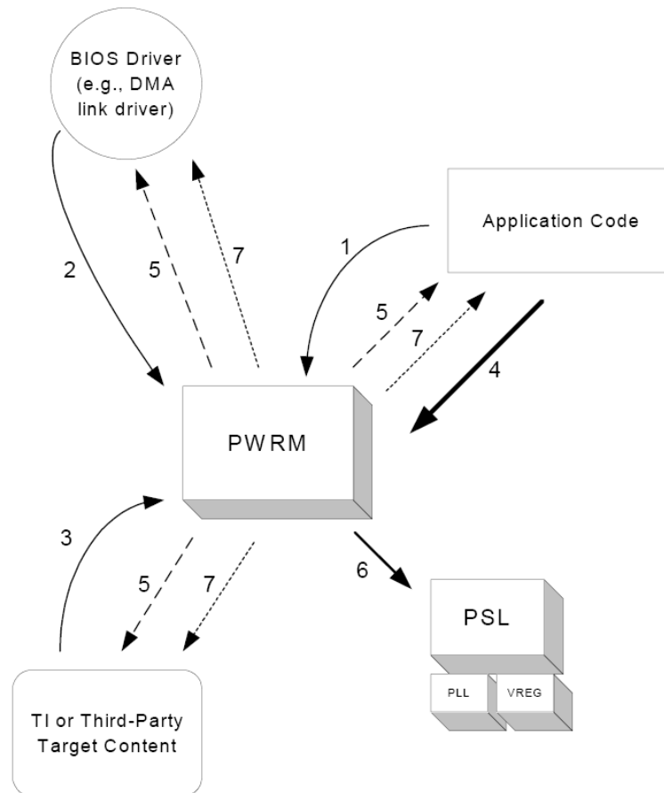
Figure 4–13 Power Event Notification
