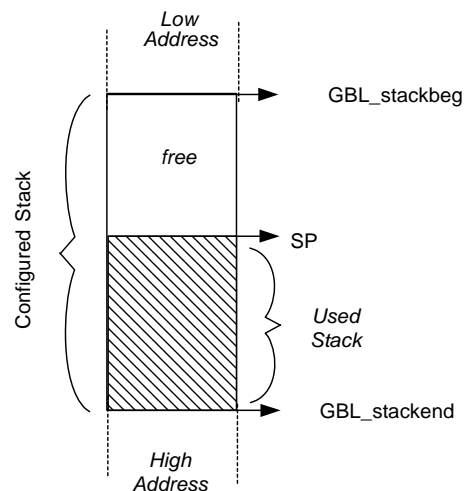
Figure 3–7 Calculating Used Stack Depth
