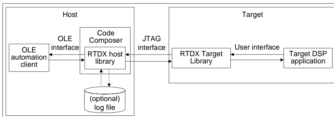
Figure 3–8 RTDX Data Flow between Host and Target
