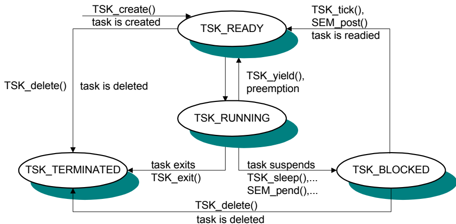
Figure 4-9. Execution Mode Variations
