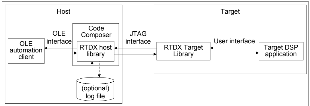
Figure 3-26. RTDX Data Flow between Host and Target
