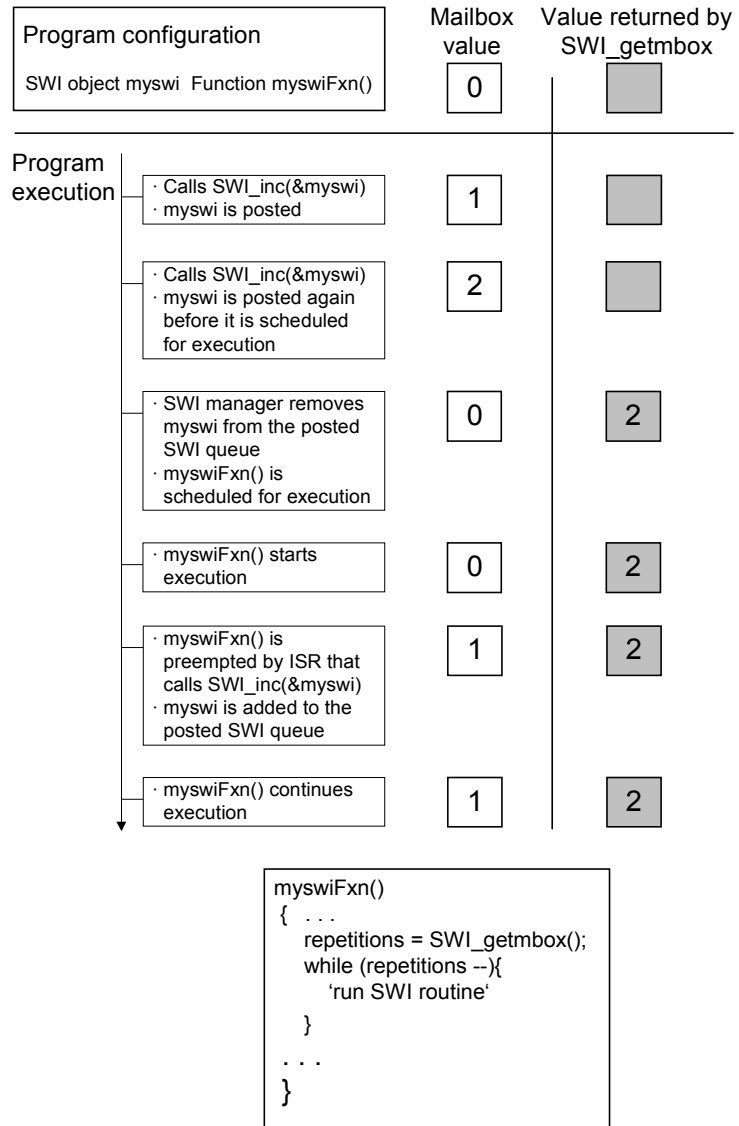
Figure 4-5. Using SWI_inc to Post an SWI
