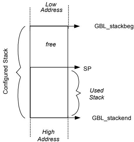
Figure 3-12. Calculating Used Stack Depth
