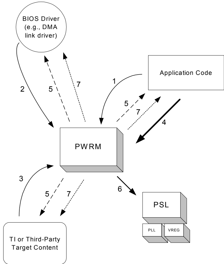
Figure 4-12. Power Event Notification
