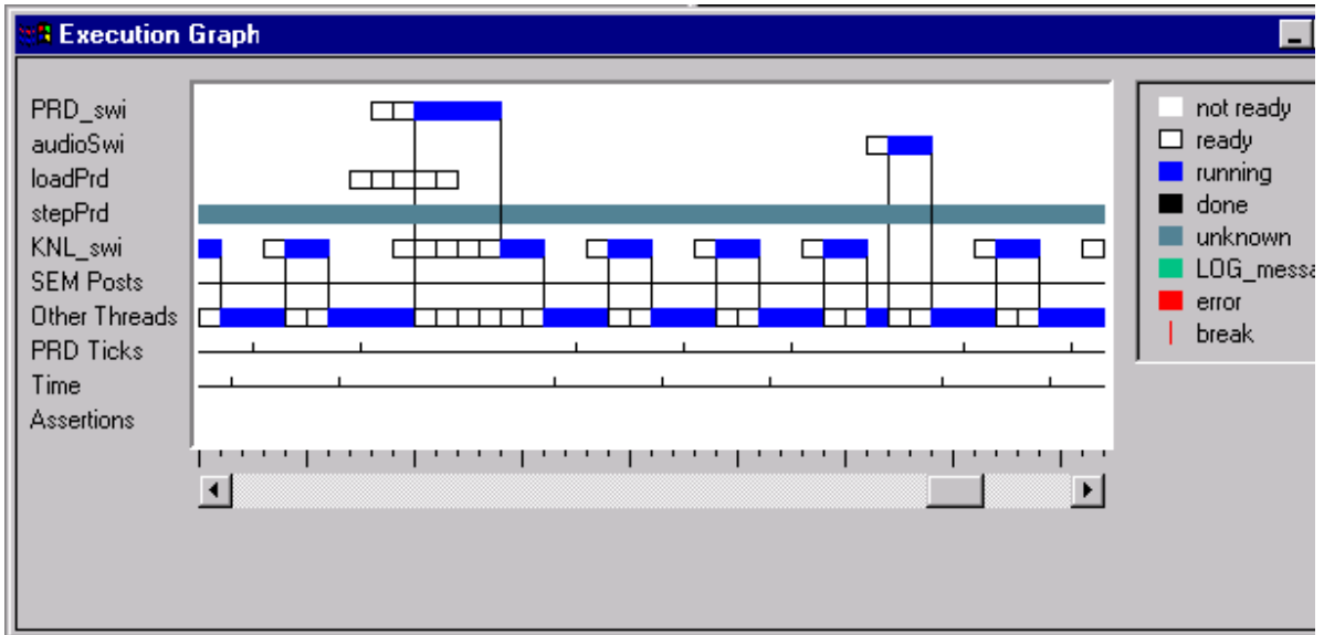
Figure 4-18. The Execution Graph Window
