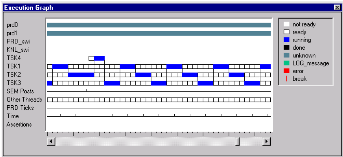
Figure 4-11. Execution Graph for Example 4-8
