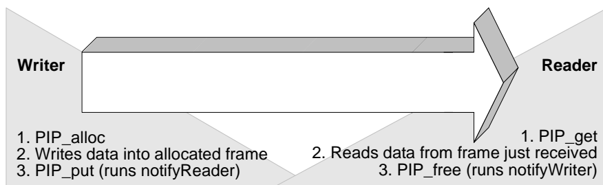
Figure 2-7. Pipe Schematic
