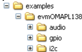
Figure 3: OMAPL138 PSP driver sample application directory structure evmOMAPL138
