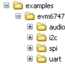
Figure 3: OMAPL137 PSP driver sample application directory structure evmOMAPL137
