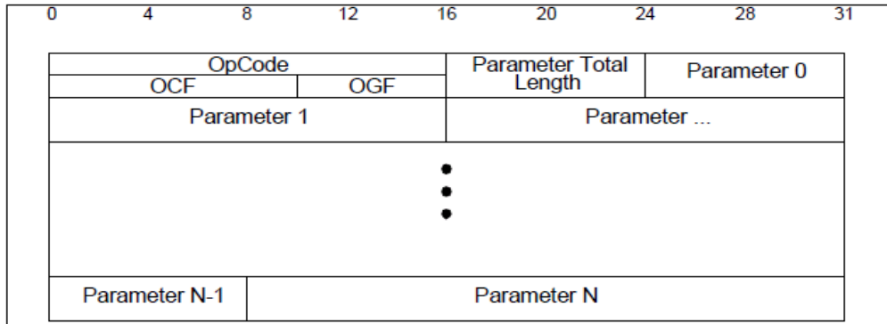
Figure 5: Command Packet
