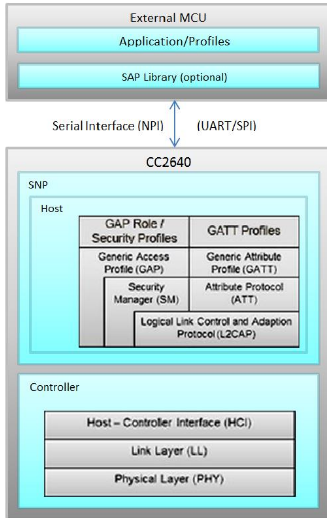
Figure 1: BLE Stack AP / NP separation
