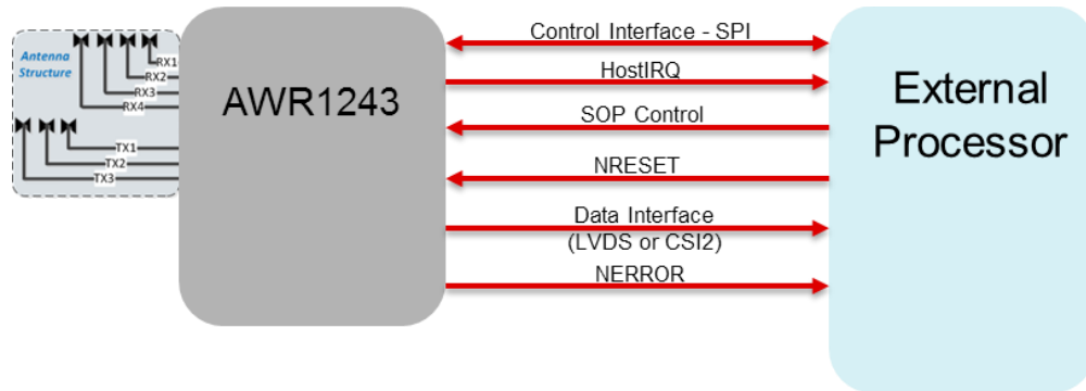
Figure 3. Connection between External Processor and AWR1243
