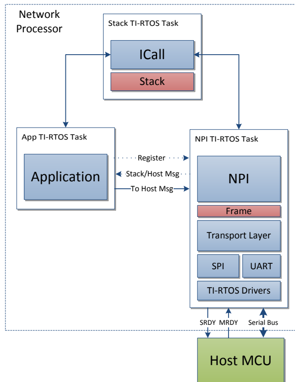
Figure 1: Network Processor Interface Framework
