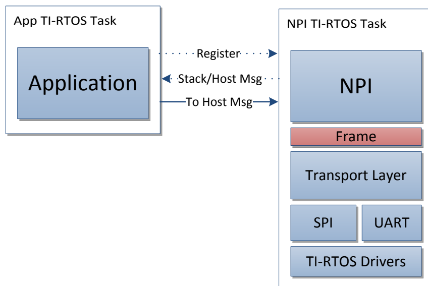
Figure 10: NPI and Application Interface
