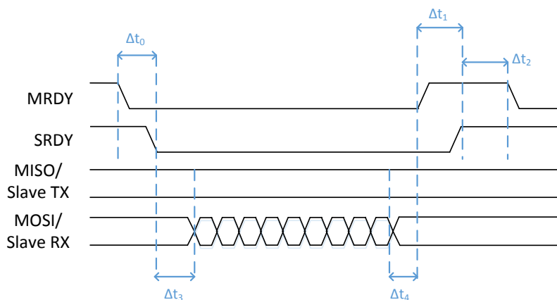
Figure 3: AREQ Timing Diagram
