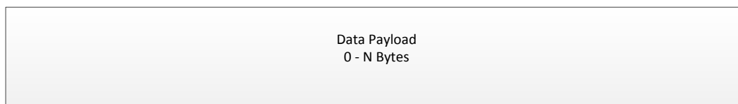
Figure 8: NPI UART Frame Format
