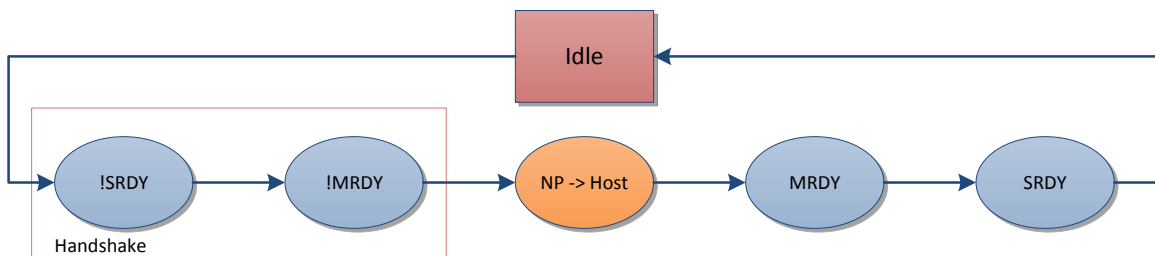
Figure 4: AIND Order of Events
