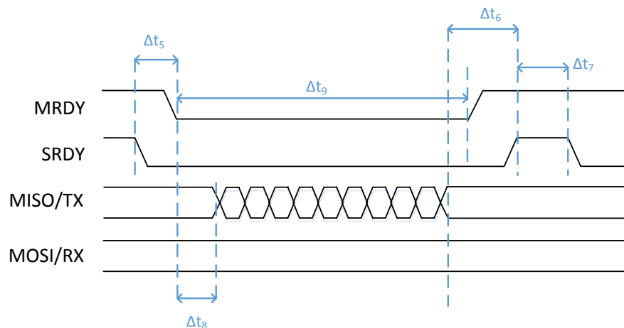
Figure 5: AIND Timing Diagram
