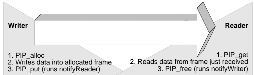
Figure 2-4. Pipe Schematic
