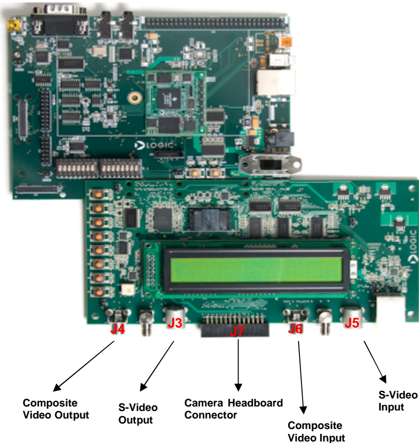
Figure 9. OMAPL138 Video Input/Output connectors Layout
