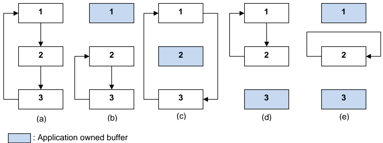
Figure 5. Capture Driver Buffer Management
