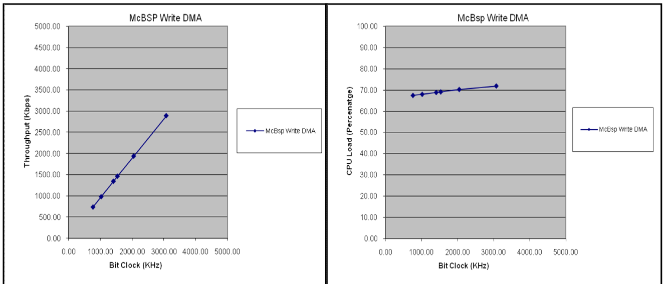
Fig: Write performance
