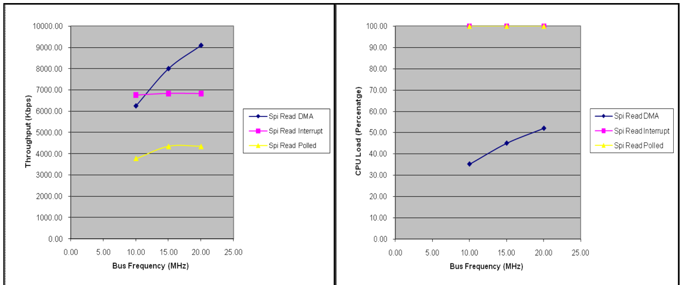
Fig: Read performance
