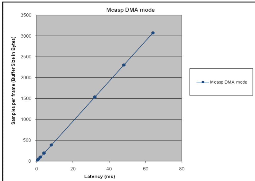
Fig: Sample size v/s Latency
