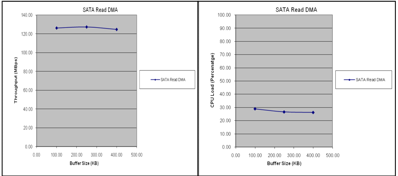
Fig: Read performance
