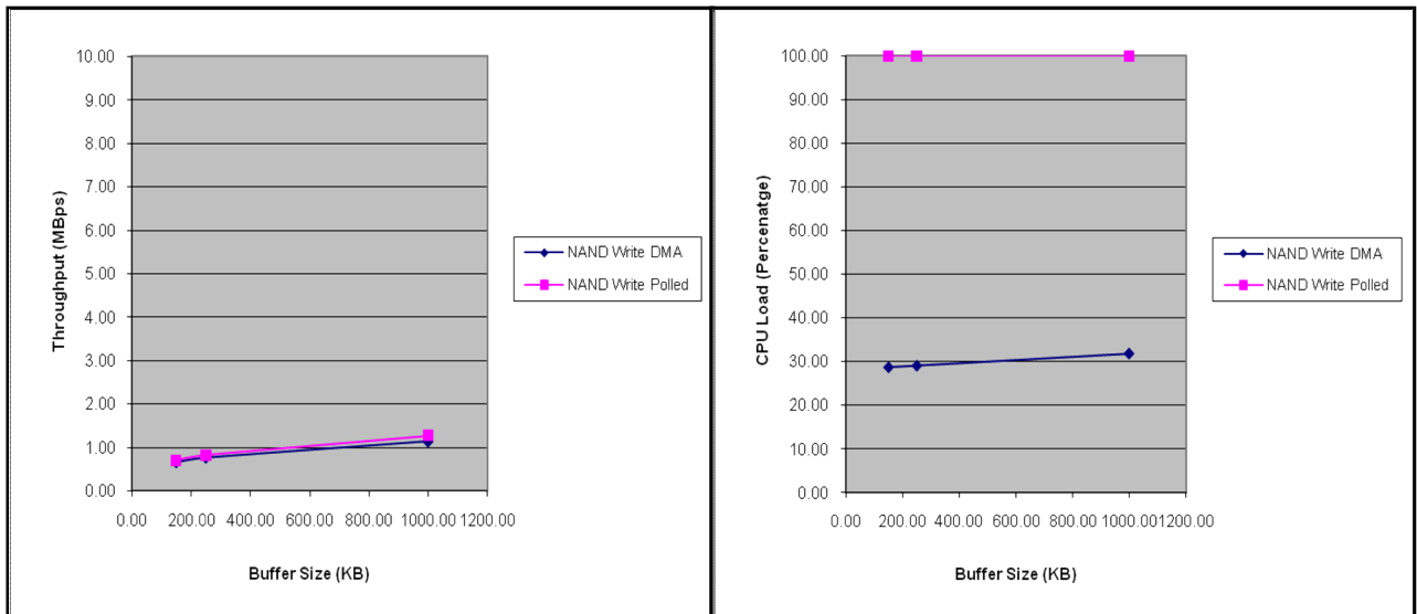
Fig: Write performance
